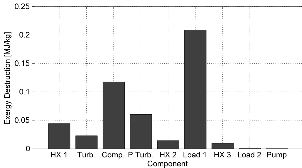
Figure 47: Intensive Exergy Destruction Thermal Management Distribution.
