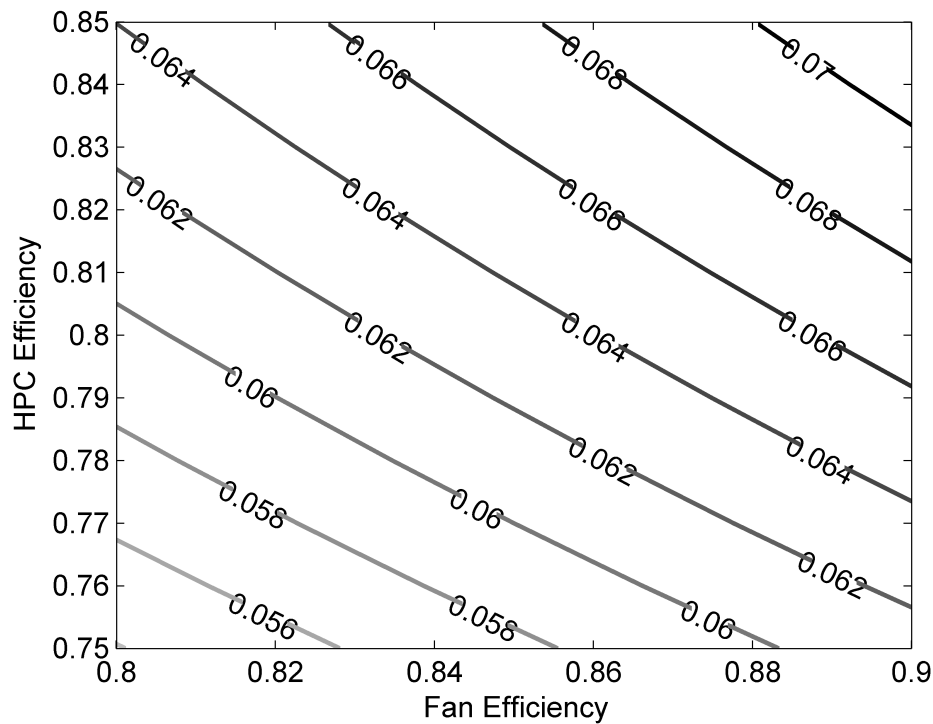
Figure 26: Isolated Engine Overall Efficiency.
