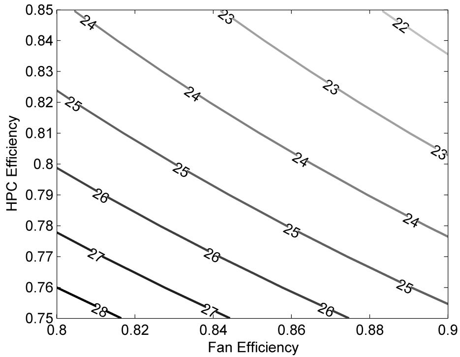
Figure 24: Isolated Engine Thrust Specific Fuel Consumption [ mg/s/N ].
