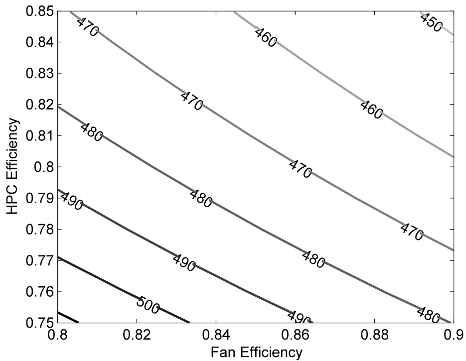
Figure 25: Isolated Engine Specific Thrust [ N/(kg/s) ].
