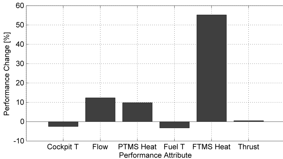
Figure 100: Performance Improvements Purchase Options Available for 500 kW of Additional Irreversibility.
