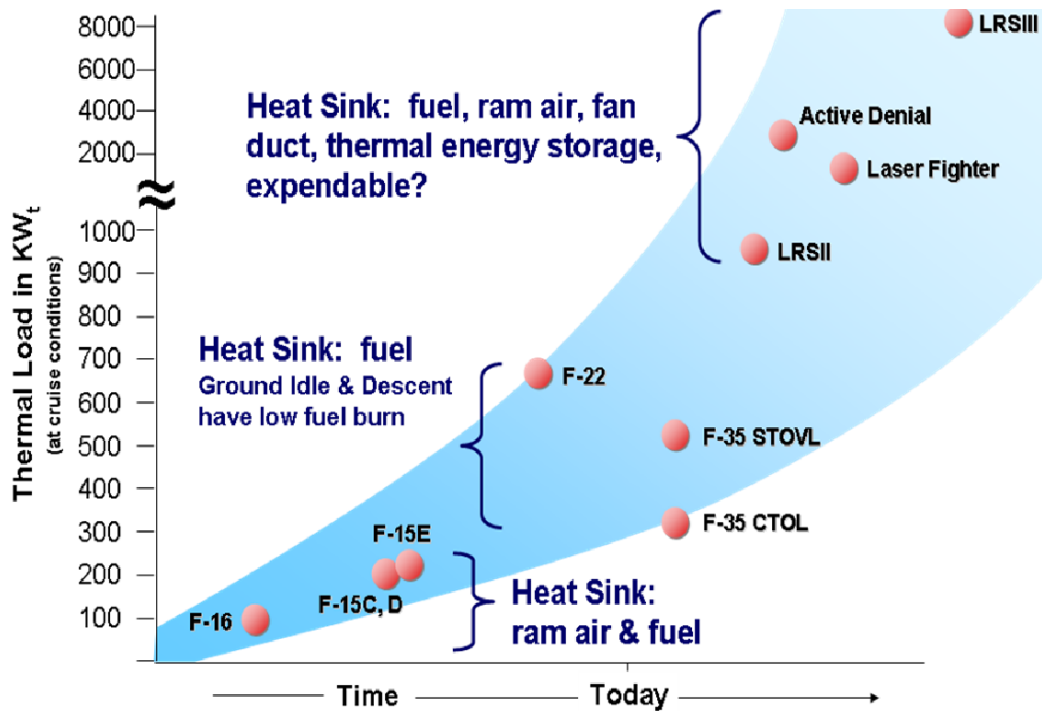
Figure 3: Thermal Load Rise for Military Aircraft Platforms [76].
