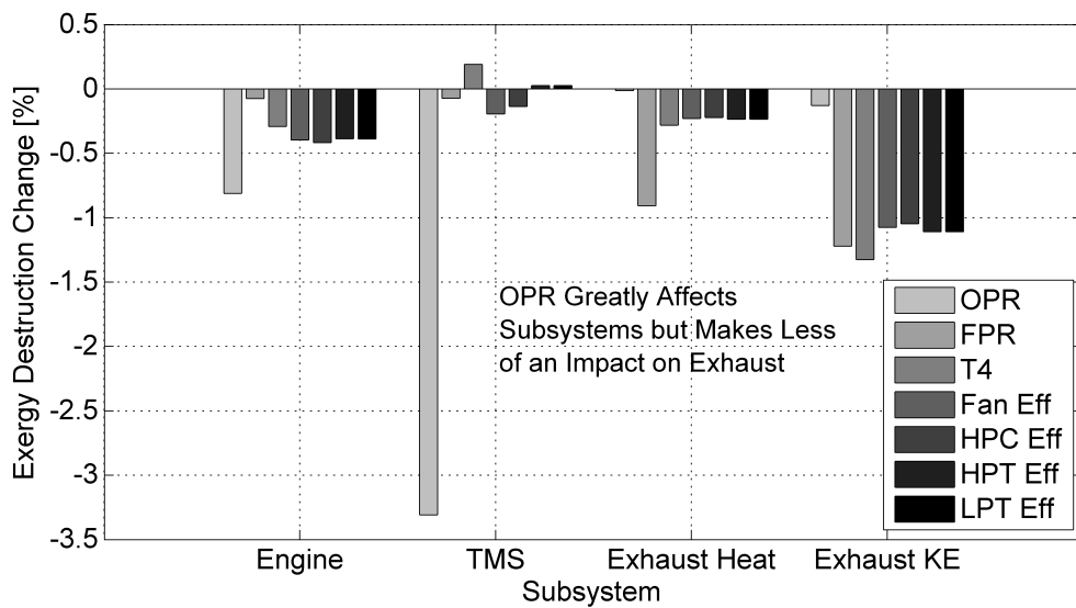
Figure 93: Changes in System Irreversibility Allocation for Sell Options.
